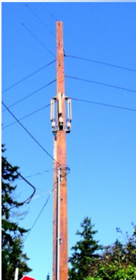
71' Distribution Structure with Flush-mounted Antennas
